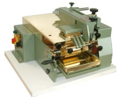
Two roller edge gluer Mod. CORONEL 90 mm
